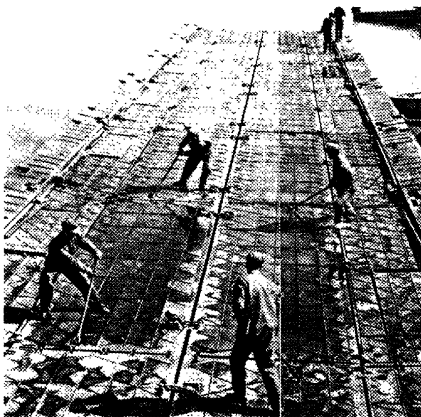
Setting Up a Pontoon Bridge.
